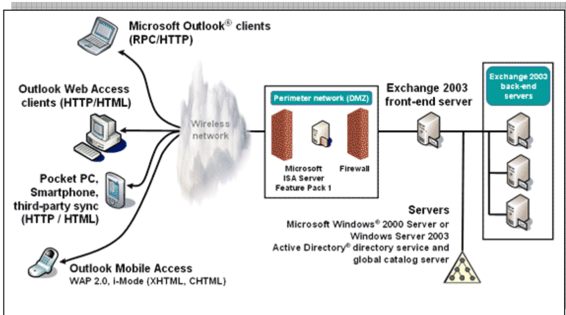
Microsoft Diagram depicts remote connectivity architecture available with Exchange.
